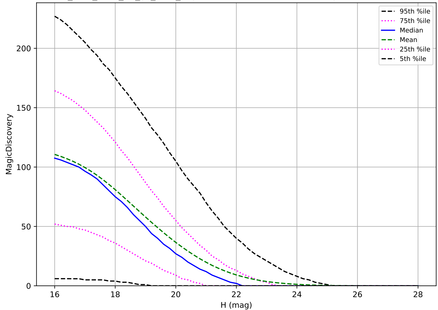
too_elab_r128_d2_gz_v3.4_10yrs: NEO 6 detections in 60 nights detection loss
