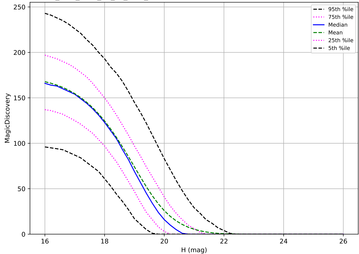
too_elab_r128_d2_gz_v3.4_10yrs: MBA 6 detections in 60 nights detection loss
