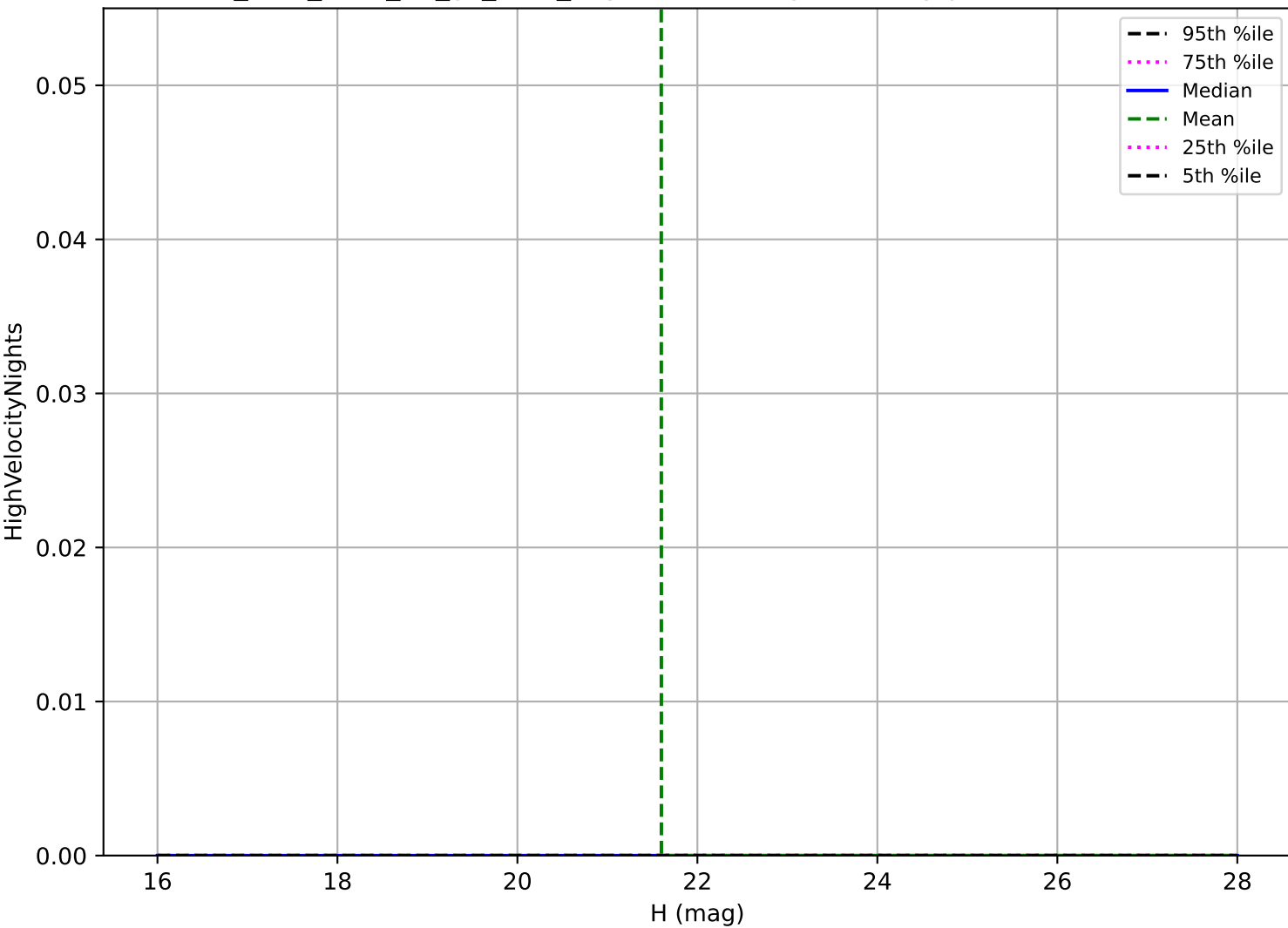
too_elab_r128_d2_gz_v3.4_10yrs: Vatira High velocity pair detection loss
