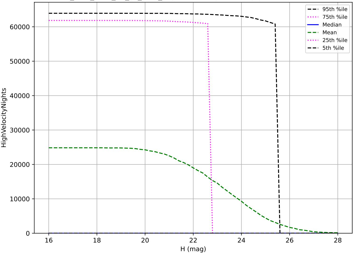
too_elab_r128_d2_gz_v3.4_10yrs: PHA High velocity pair detection loss
