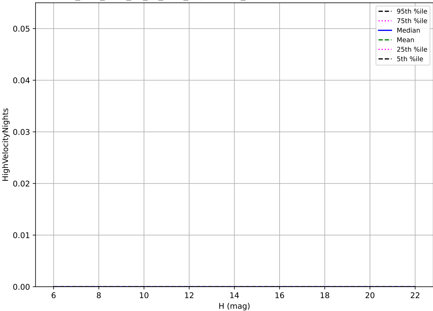
too_elab_r128_d2_gz_v3.4_10yrs: OCC_r5 High velocity pair detection loss
