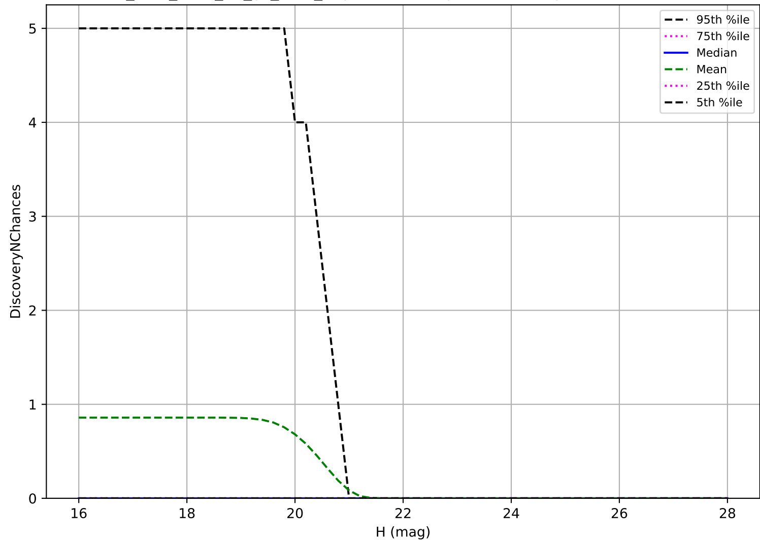
too_elab_r128_d2_gz_v3.4_10yrs: Vatira 3 pairs in 15 nights detection loss
