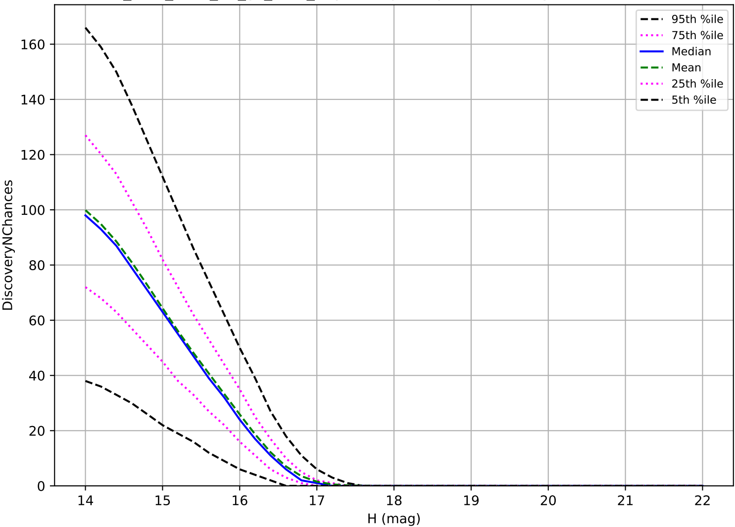
too_elab_r128_d2_gz_v3.4_10yrs: Trojan 3 pairs in 15 nights detection loss
