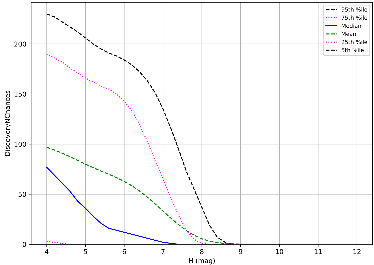
too_elab_r128_d2_gz_v3.4_10yrs: TNO 3 pairs in 15 nights detection loss
