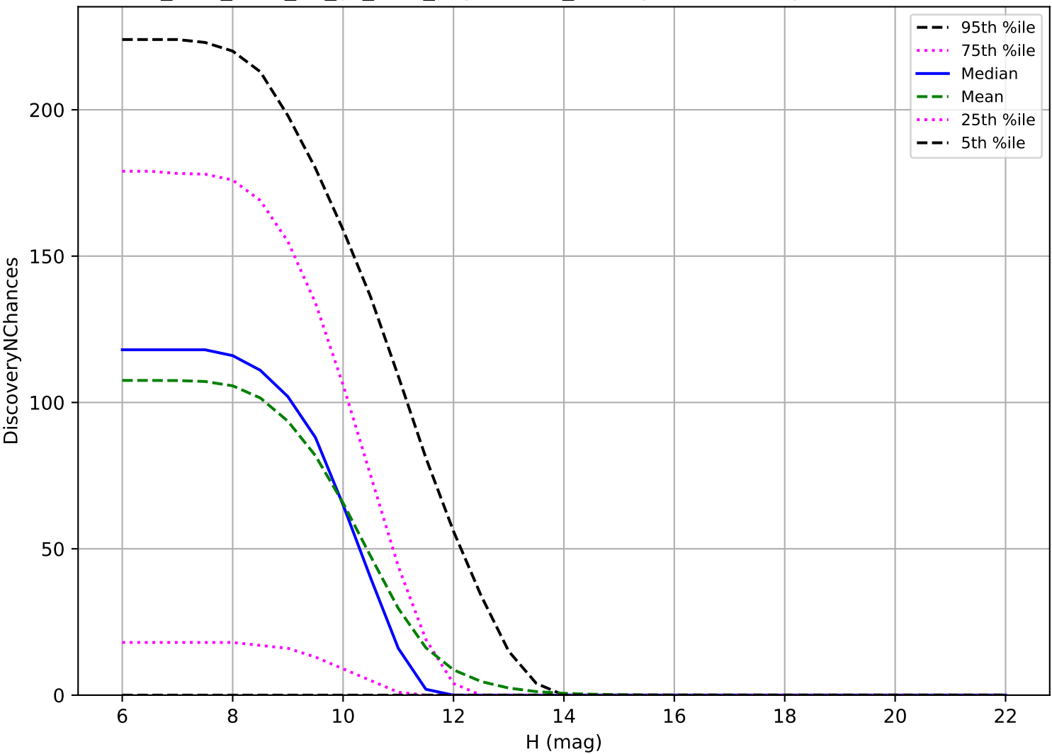
too_elab_r128_d2_gz_v3.4_10yrs: OCC_r20 3 pairs in 15 nights detection loss
