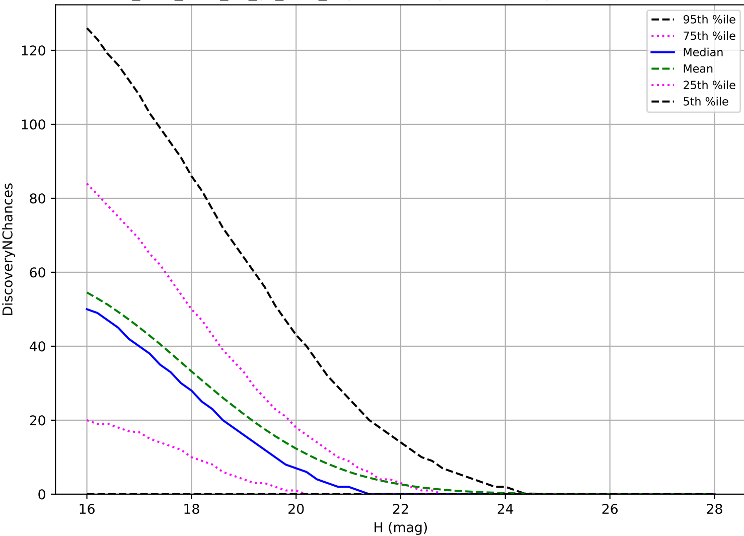
too_elab_r128_d2_gz_v3.4_10yrs: NEO 3 pairs in 15 nights detection loss
