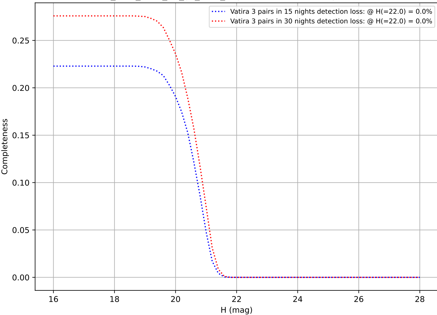
too_elab_r128_d2_gz_v3.4_10yrs: DifferentialCompleteness
