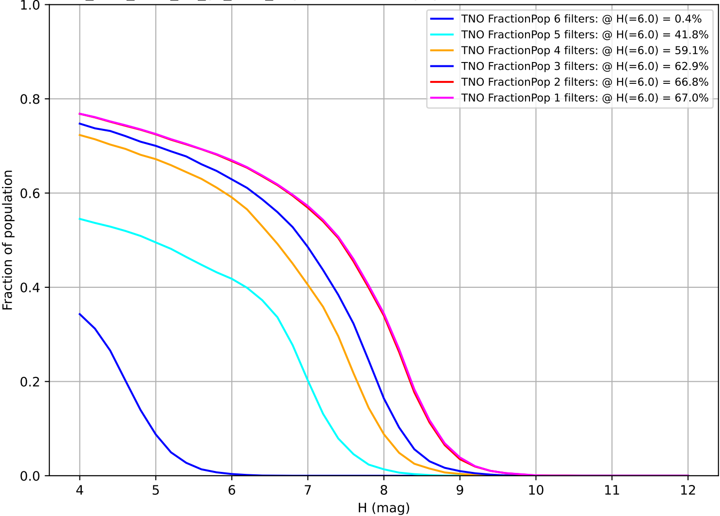
too_elab_r128_d2_gz_v3.4_10yrs: Fraction of population with colors in X filters TNO
