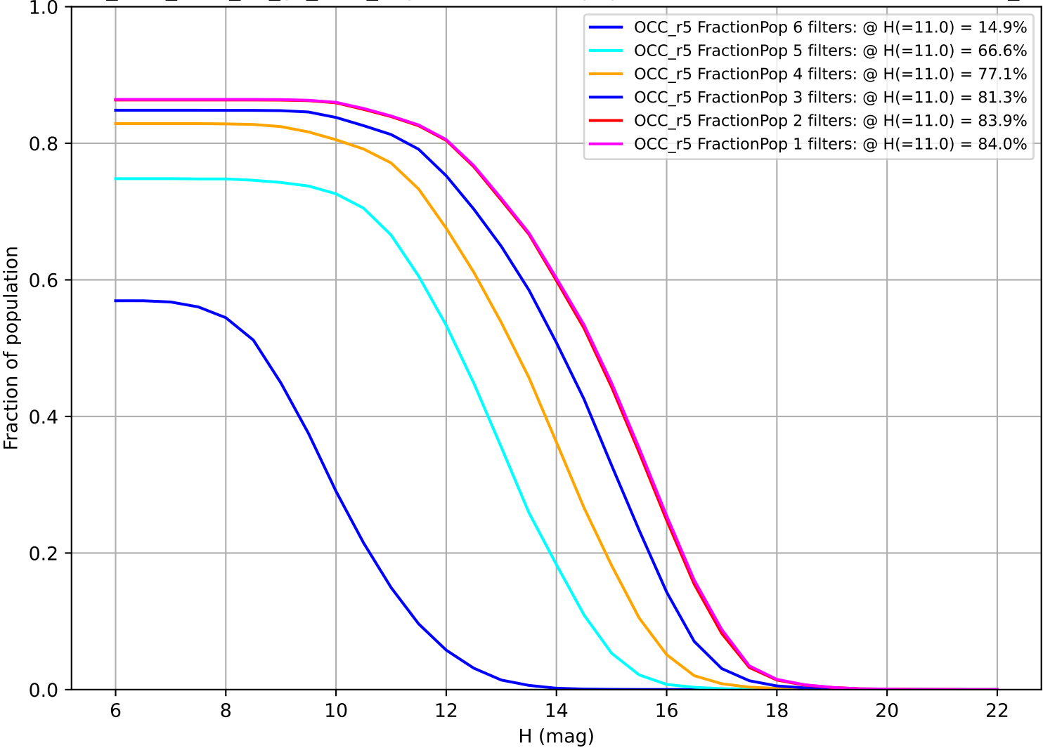
too_elab_r128_d2_gz_v3.4_10yrs: Fraction of population with colors in X filters OCC_r5
