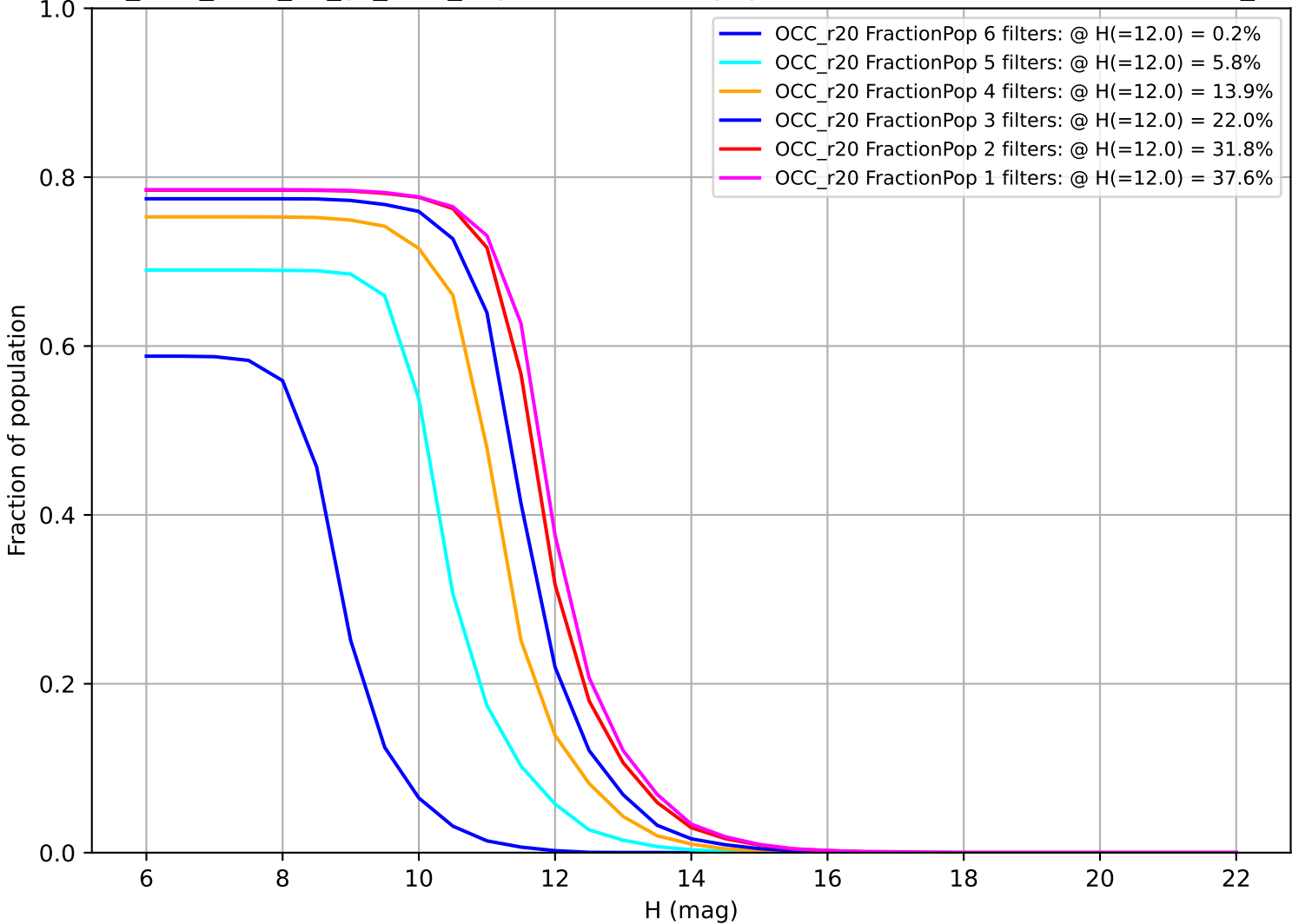
too_elab_r128_d2_gz_v3.4_10yrs: Fraction of population with colors in X filters OCC_r20
