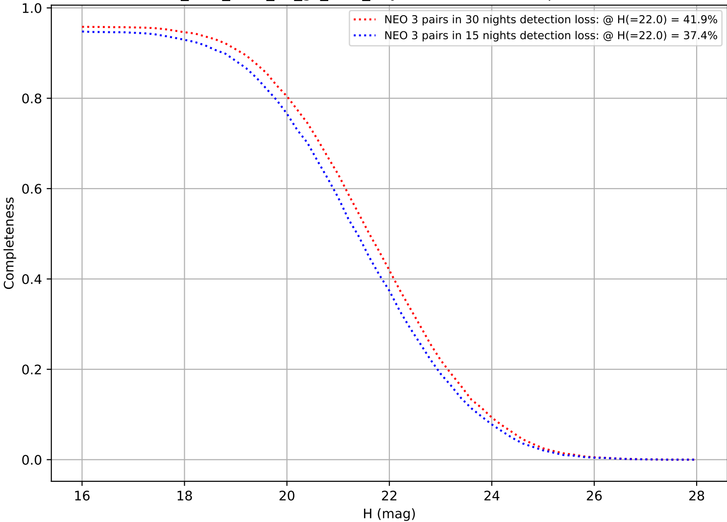
too_elab_r128_d2_gz_v3.4_10yrs: DifferentialCompleteness
