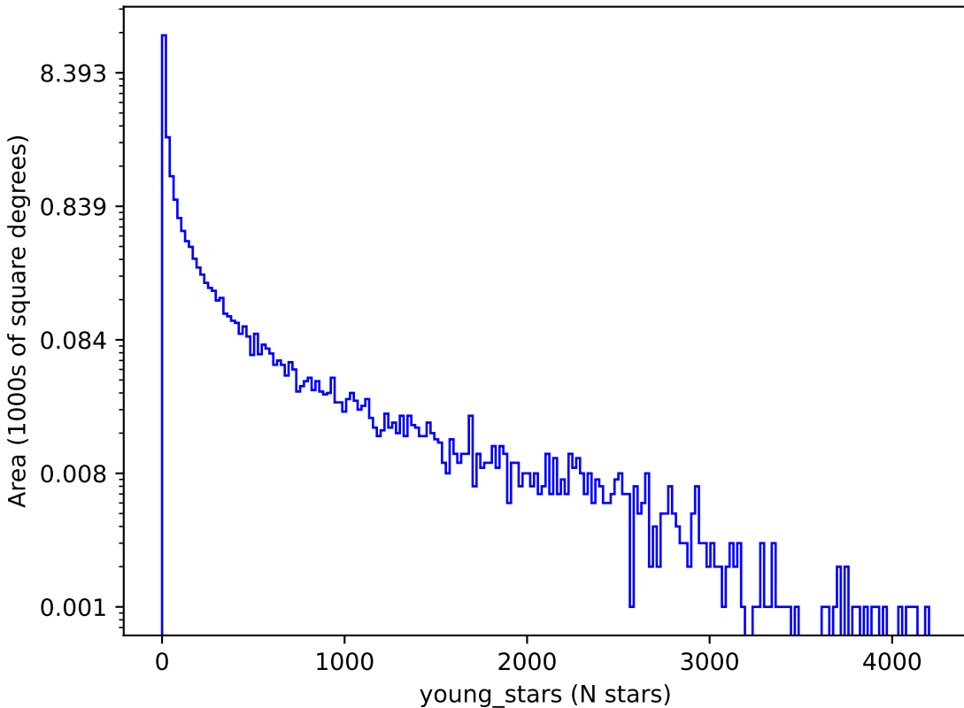
too_elab_r128_d2_gz_v3.4_10yrs : young_stars
