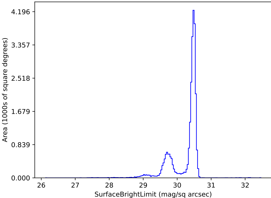
too_elab_r128_d2_gz_v3.4_10yrs r: SurfaceBrightLimit
