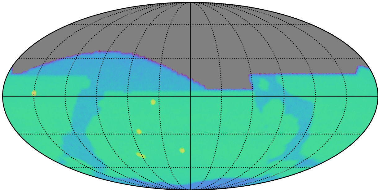
too_elab_r128_d2_gz_v3.4_10yrs i: SurfaceBrightLimit
