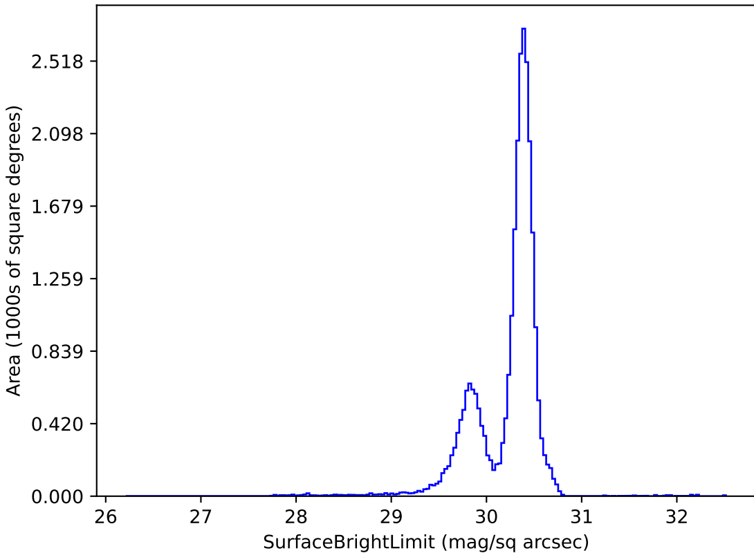
too_elab_r128_d2_gz_v3.4_10yrs g: SurfaceBrightLimit
