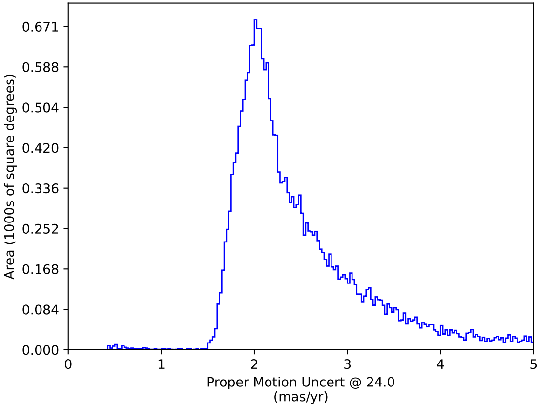
too_elab_r128_d2_gz_v3.4_10yrs : Proper Motion Uncert @ 24.0
