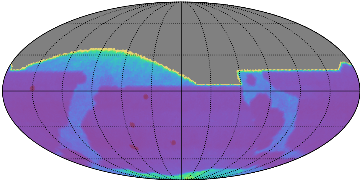
too_elab_r128_d2_gz_v3.4_10yrs : Proper Motion Uncert @ 20.5
