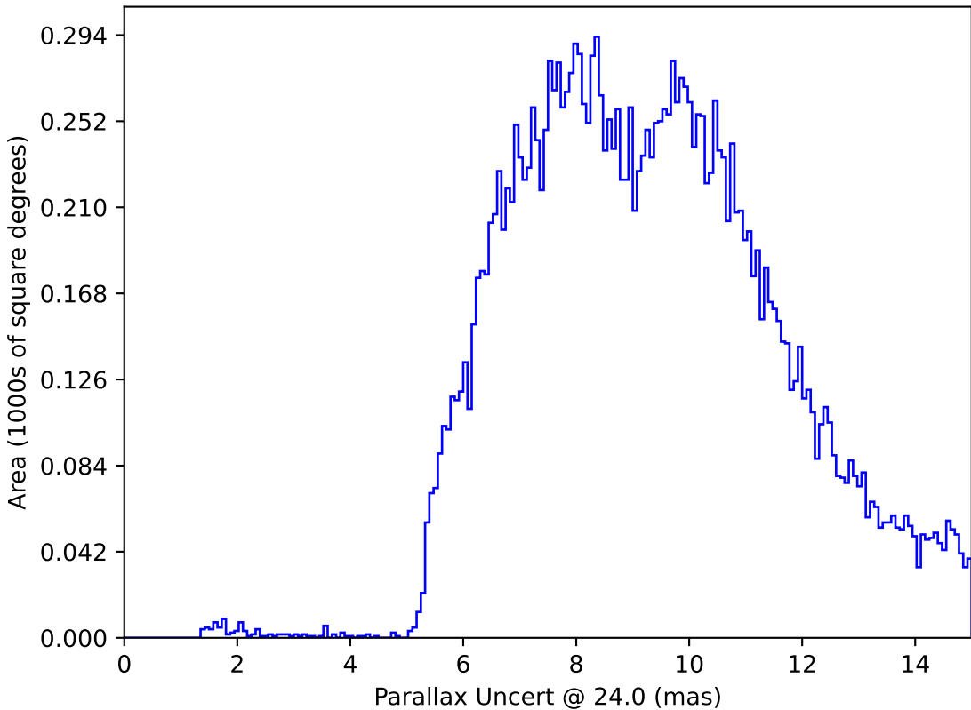
too_elab_r128_d2_gz_v3.4_10yrs : Parallax Uncert @ 24.0
