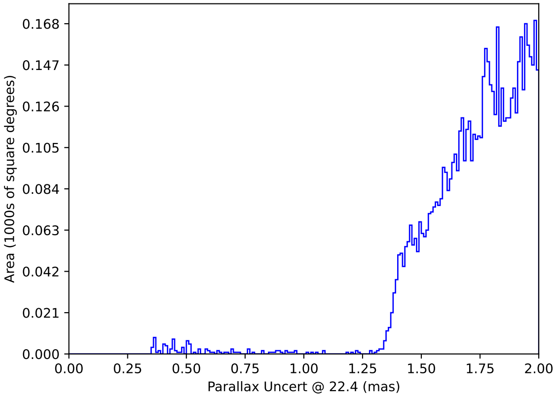
too_elab_r128_d2_gz_v3.4_10yrs : Parallax Uncert @ 22.4
