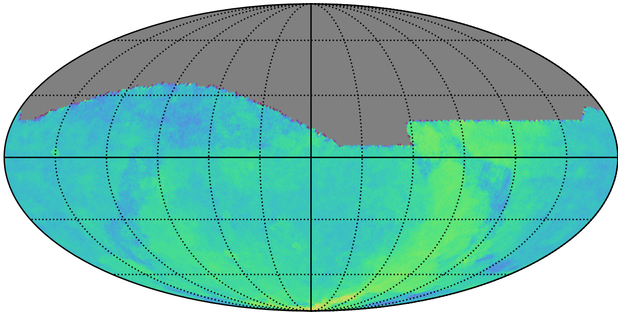
too_elab_r128_d2_gz_v3.4_10yrs : Parallax Coverage @ 22.4
