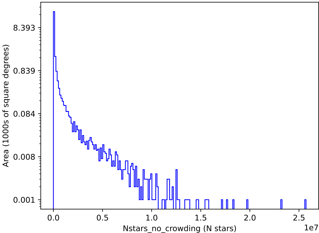
too_elab_r128_d2_gz_v3.4_10yrs y: Nstars_no_crowding
