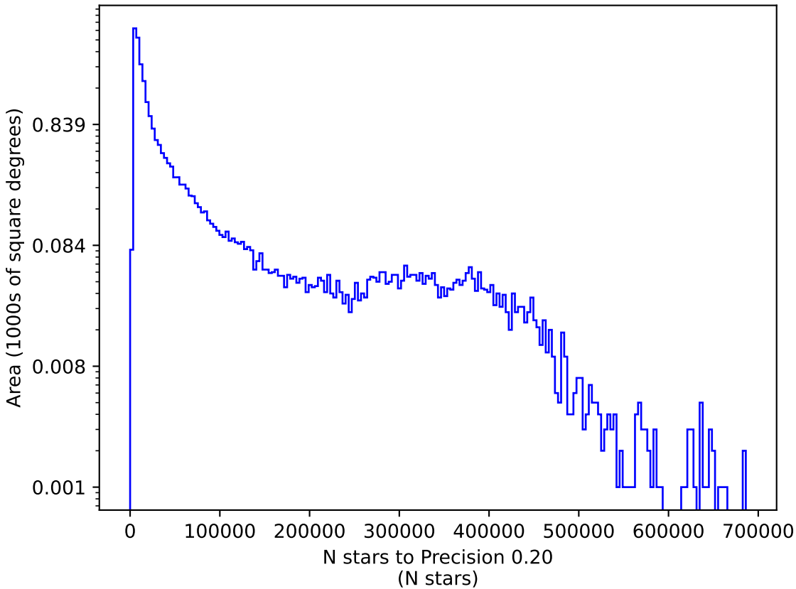
too_elab_r128_d2_gz_v3.4_10yrs g: N stars to Precision 0.20
