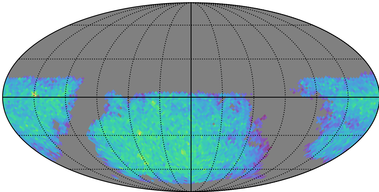
too_elab_r128_d2_gz_v3.4_10yrs gi: LVDwarfs
