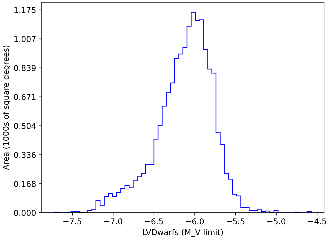
too_elab_r128_d2_gz_v3.4_10yrs gi: LVDwarfs
