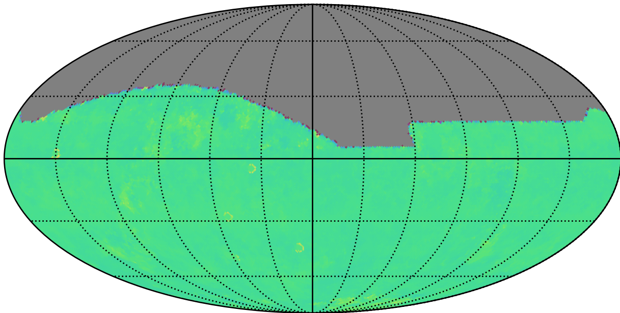
too_elab_r128_d2_gz_v3.4_10yrs z: Kuiper rotTelPos
