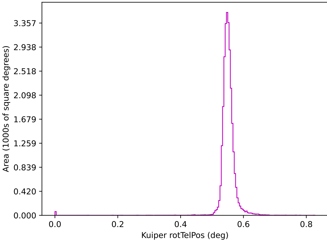
too_elab_r128_d2_gz_v3.4_10yrs z: Kuiper rotTelPos
