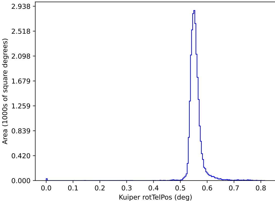
too_elab_r128_d2_gz_v3.4_10yrs y: Kuiper rotTelPos
