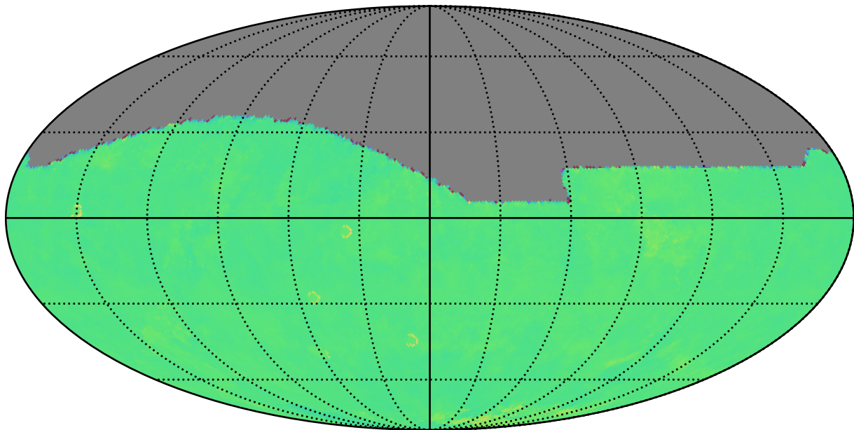
too_elab_r128_d2_gz_v3.4_10yrs r: Kuiper rotTelPos
