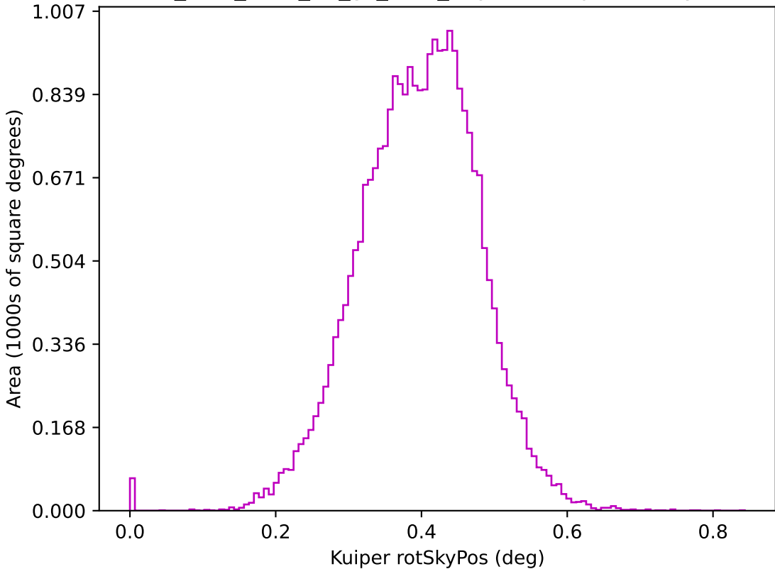
too_elab_r128_d2_gz_v3.4_10yrs z: Kuiper rotSkyPos
