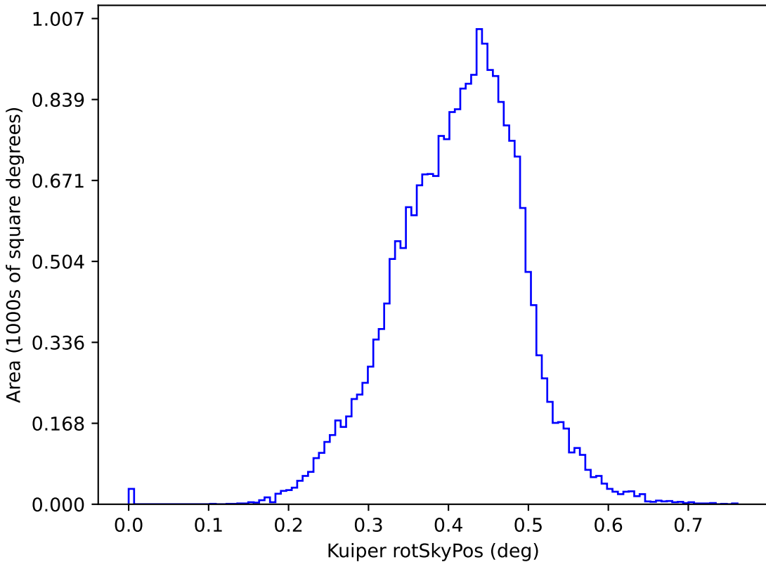
too_elab_r128_d2_gz_v3.4_10yrs y: Kuiper rotSkyPos
