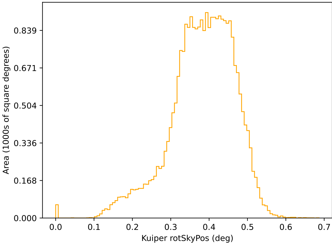
too_elab_r128_d2_gz_v3.4_10yrs r: Kuiper rotSkyPos
