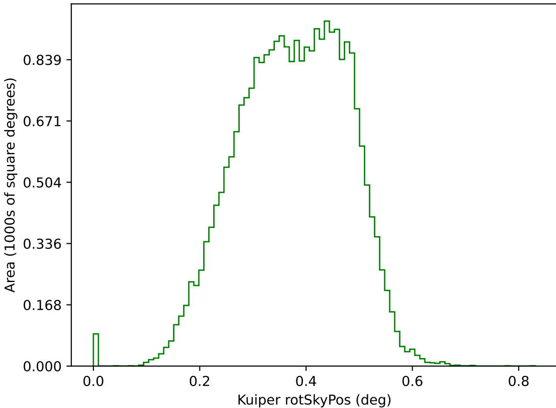
too_elab_r128_d2_gz_v3.4_10yrs g: Kuiper rotSkyPos
