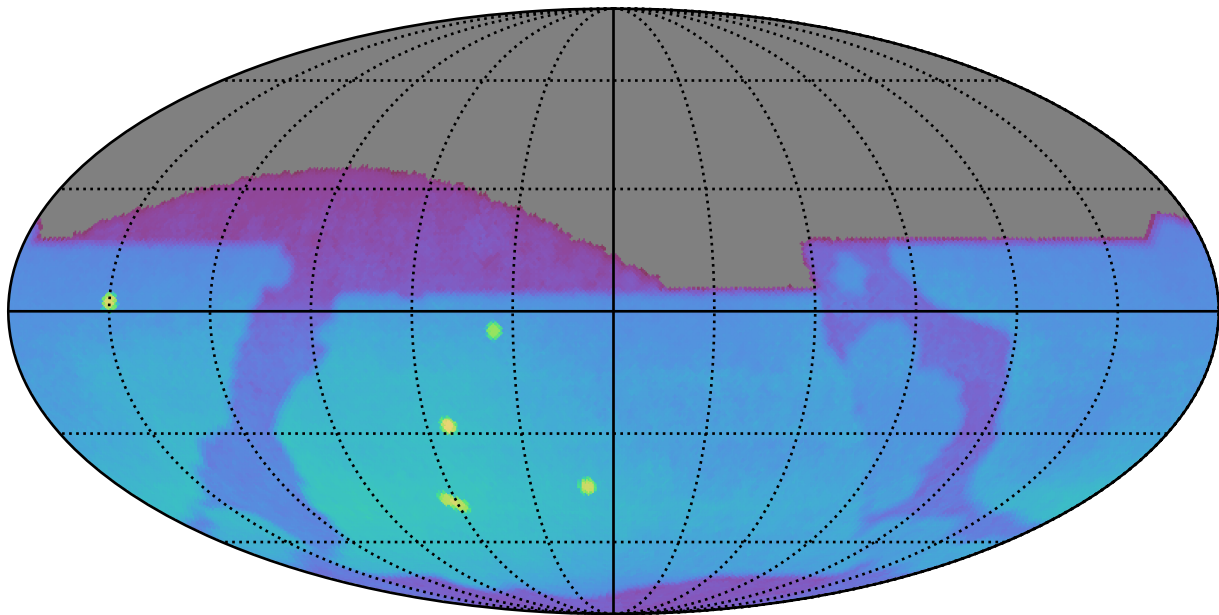
too_elab_r128_d2_gz_v3.4_10yrs : Brown Dwarf, L7
