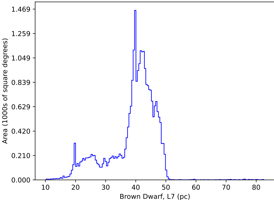
too_elab_r128_d2_gz_v3.4_10yrs : Brown Dwarf, L7
