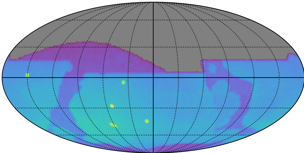
too_elab_r128_d2_gz_v3.4_10yrs : Brown Dwarf, L4
