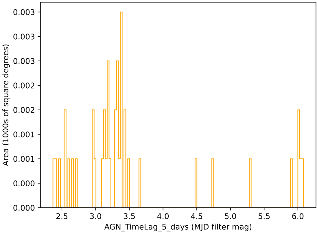
too_elab_r128_d2_gz_v3.4_10yrs r band: AGN_TimeLag_5_days
