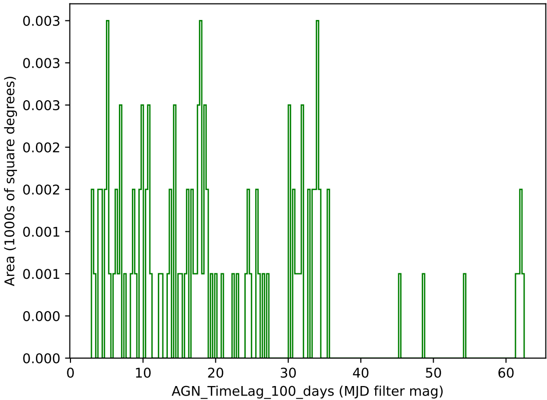
too_elab_r128_d2_gz_v3.4_10yrs g band: AGN_TimeLag_100_days
