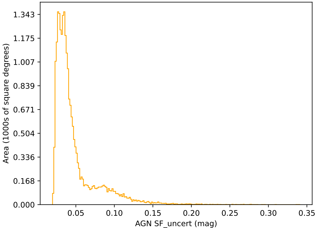
too_elab_r128_d2_gz_v3.4_10yrs r band: AGN SF_uncert
