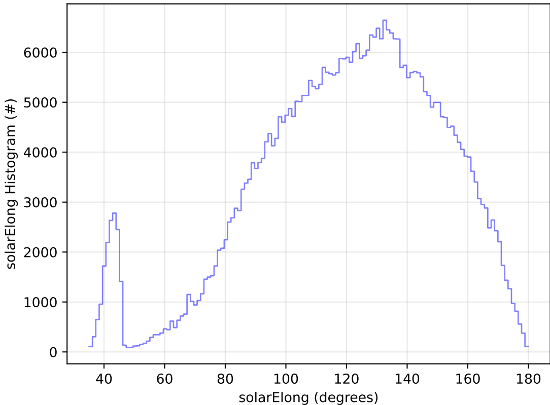
too_elab_r128_d2_gz_v3.4_10yrs WFD z band: solarElong Histogram
