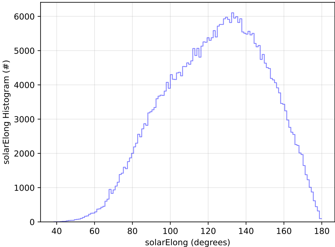
too_elab_r128_d2_gz_v3.4_10yrs WFD y band: solarElong Histogram
