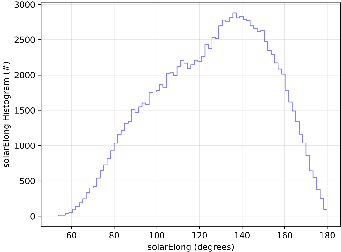
too_elab_r128_d2_gz_v3.4_10yrs WFD u band: solarElong Histogram
