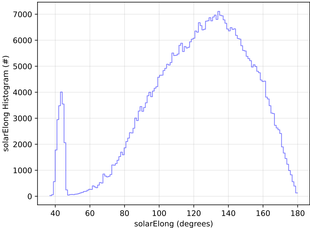
too_elab_r128_d2_gz_v3.4_10yrs WFD r band: solarElong Histogram
