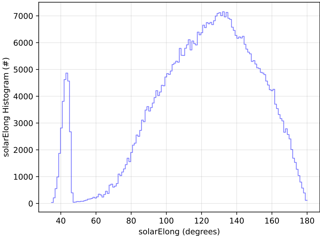
too_elab_r128_d2_gz_v3.4_10yrs WFD i band: solarElong Histogram
