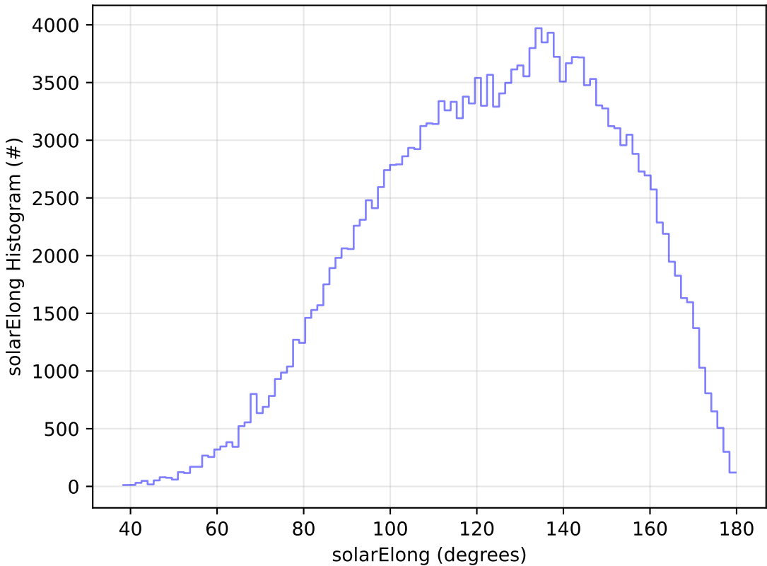
too_elab_r128_d2_gz_v3.4_10yrs WFD g band: solarElong Histogram
