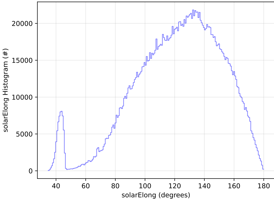
too_elab_r128_d2_gz_v3.4_10yrs WFD all bands: solarElong Histogram
