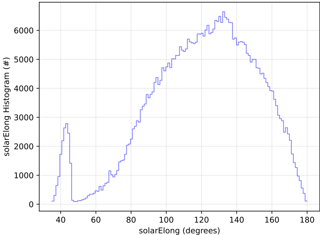
too_elab_r128_d2_gz_v3.4_10yrs All sky z band: solarElong Histogram
